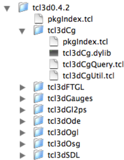
Figure 1.1: Tcl3D package layout
