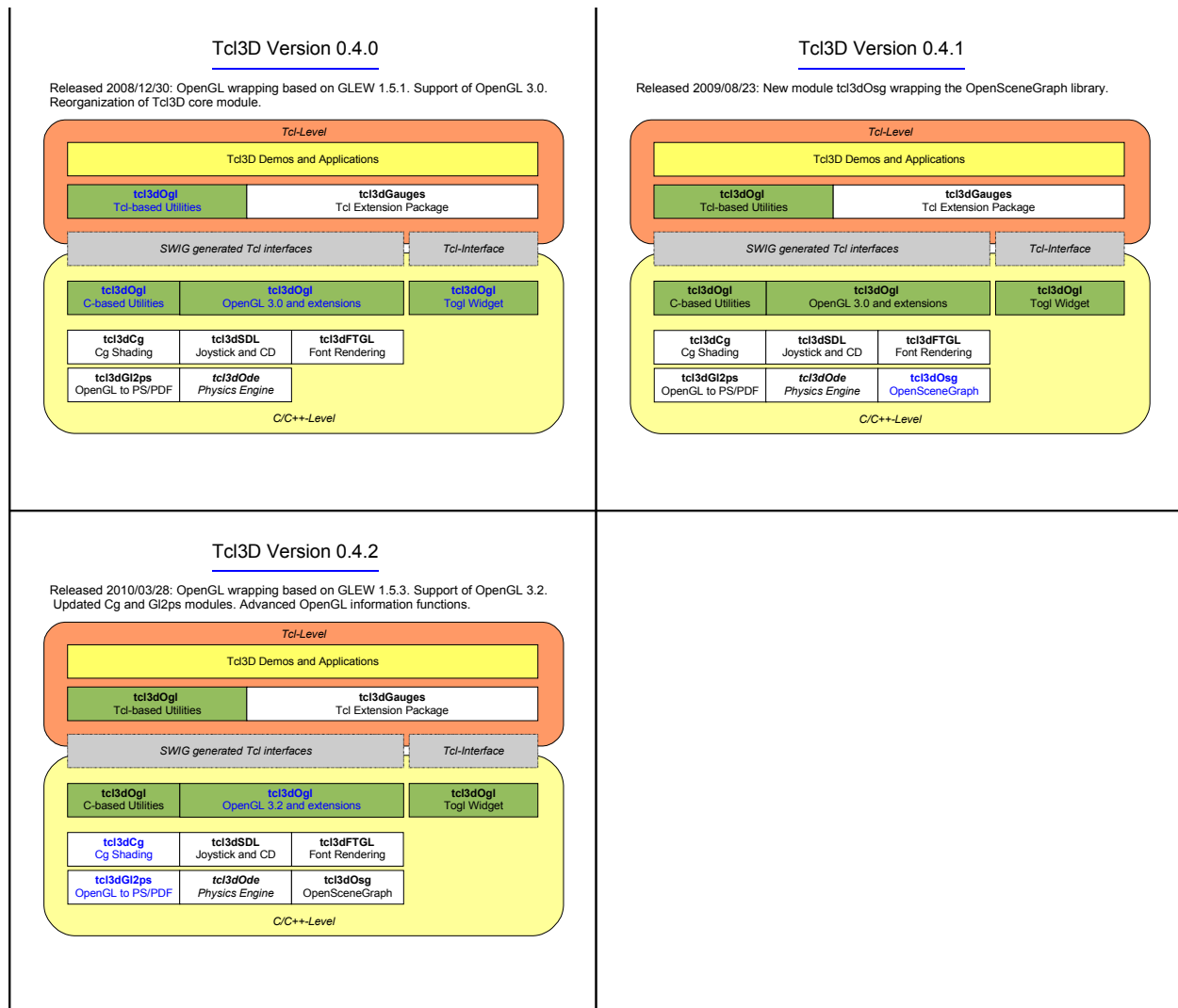
Figure 7.1: Tcl3D graphical release history
