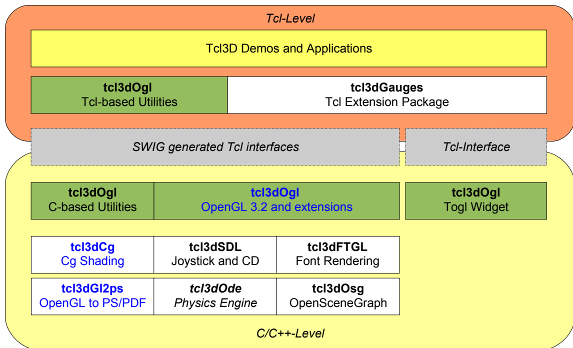
Figure 1.2: Overview of Tcl3D modules
