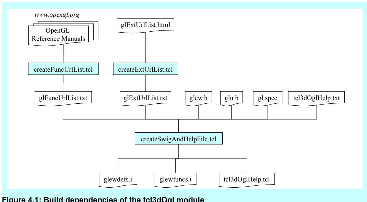
Figure 4.1: Build dependencies of the tcl3dOgl module
