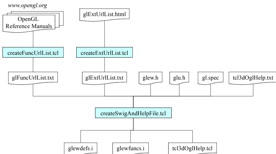
Figure 4.1: Build dependencies of the tcl3dOgl module
