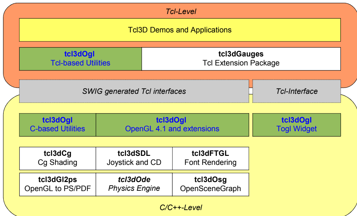
Figure 1.2: Overview of Tcl3D modules
