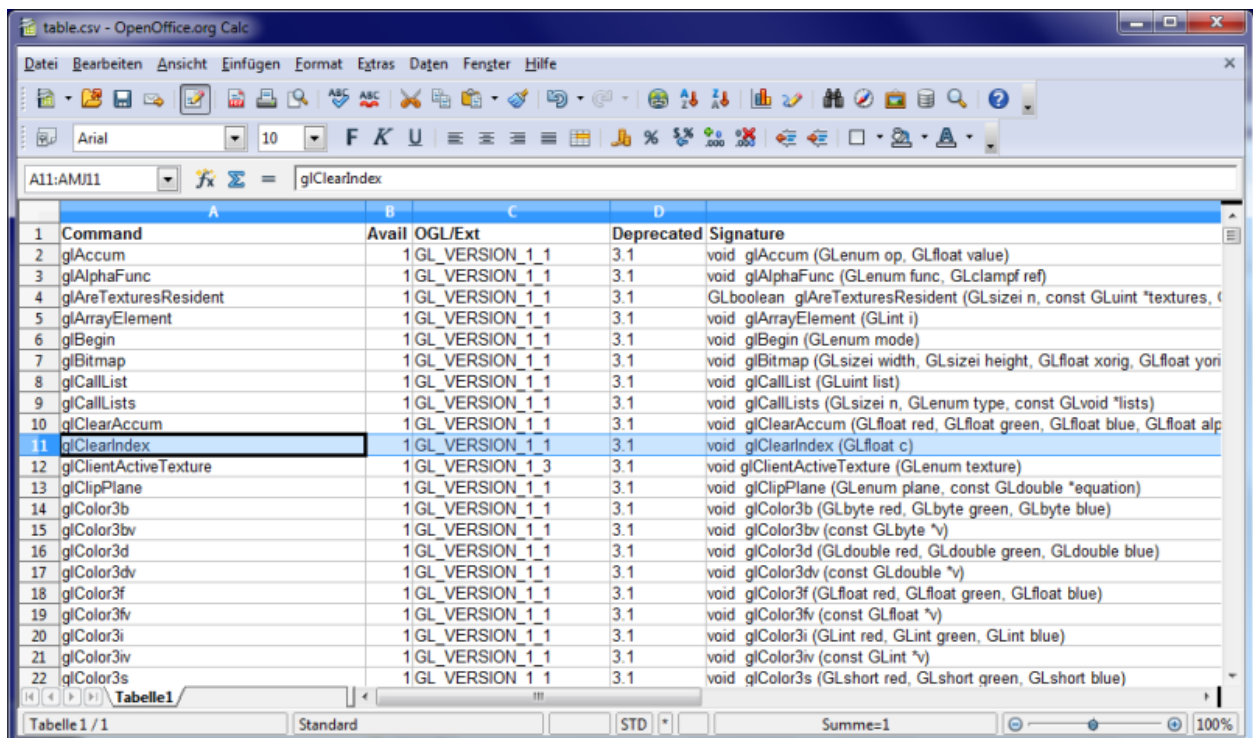
Figure 11: OglInfo export
