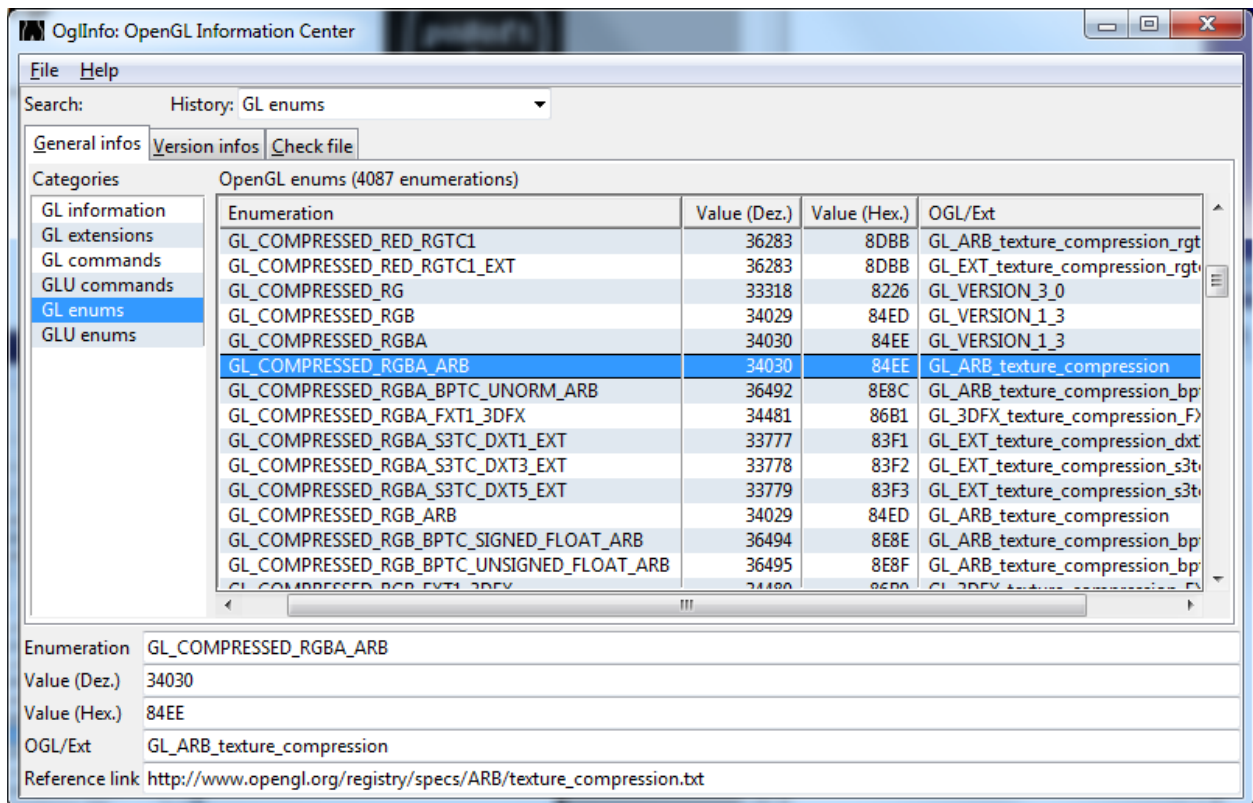
Figure 7: OglInfo category: GL enums
