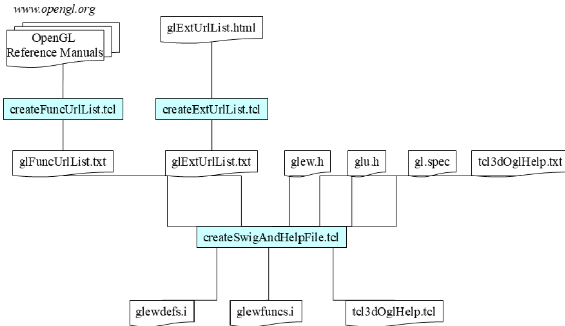
Figure 3: Build dependencies of the tcl3dOgl module
